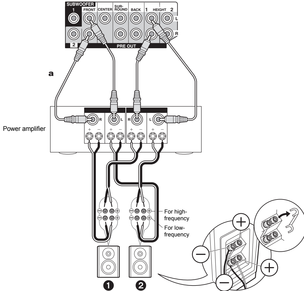
a Analog Audio Cable
