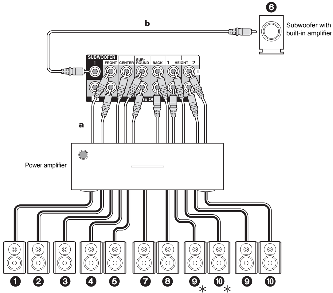
a Analog Audio Cable, b Subwoofer Cable
